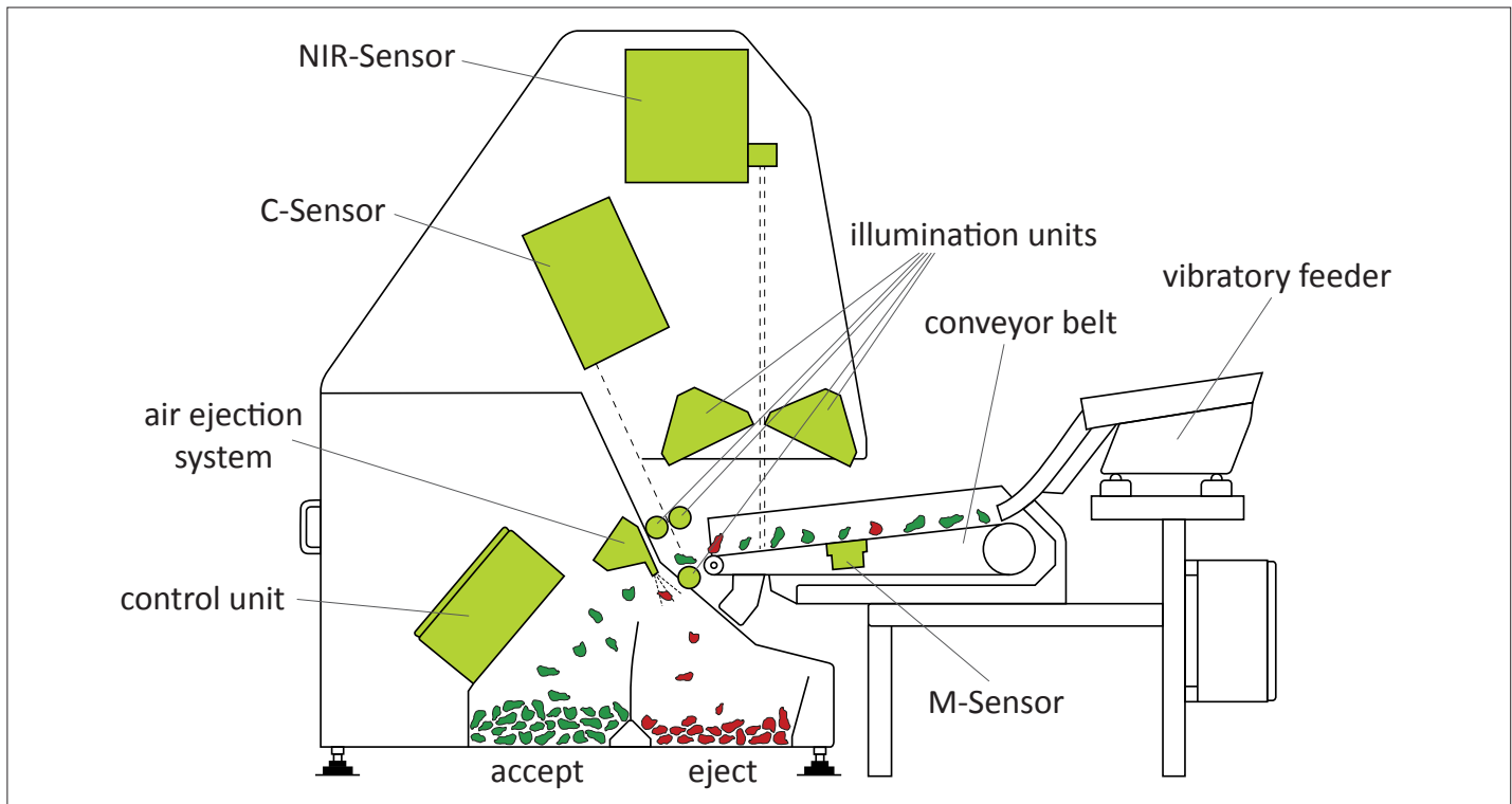
Function description: VARISORT COMPACT multi-sensor sorting machine
